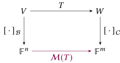
Figure 1: The matrix is the map written in coordinates: passing to coordinates and multiplying by \mathcal{M}(T) gives the same result as applying T and only then passing to coordinates.
