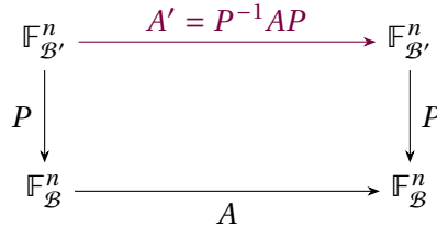
Figure 2: Similarity. To apply T in the new basis, we first convert the coordinates to the old basis ( P ), then multiply by A , and convert back to the new basis ( P^{-1} ).
