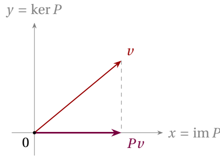
Figure 2: Projection onto the x -axis: the kernel is the y -axis, the image is the x -axis, and \dim \ker P + \dim \text{im } P = 1 + 1 = 2 .
