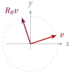
Figure 2: When \theta \notin \pi\mathbb{Z} , a rotation moves every nonzero real vector off its line, so there are no real eigenvectors.
