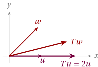
Figure 1: The eigendirection of the transformation T(x, y) = (2x, \frac{1}{2}y) is the x axis: Tu = 2u . A general vector w is turned, so it is not an eigenvector.
