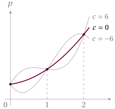
Figure 3: Three trajectories through the same three measured positions (dots): the members p(t) = p_0(t) + c t(t-1)(t-2) of the solution family for c = 0 , which is the particular solution p_0(t) = 3 + t + 2t^2 , and for c = 6 and c = -6 .
