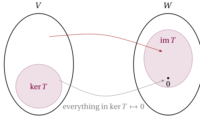
Figure 1: A linear map collapses its kernel to 0 and carries a complement of the kernel one-to-one onto its image; the dimensions balance as \dim V = \dim \ker T + \dim \text{im } T .
