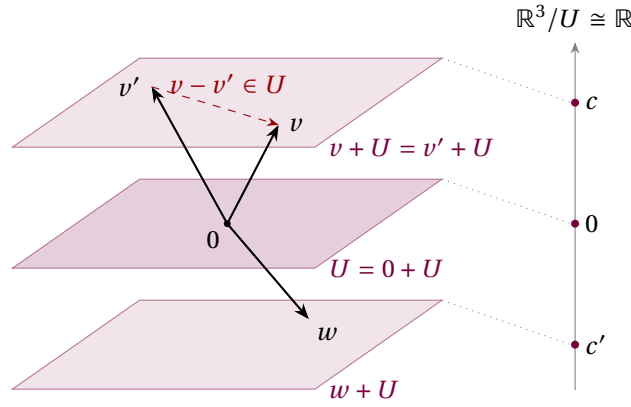
Figure 4: The cosets of the plane U in \mathbb{R}^3 are the planes parallel to it. The vectors v and v' lie in the same coset, since v - v' \in U . The coset of w is a different plane. Each plane is one element of the quotient space \mathbb{R}^3/U , and a single number identifies it: the height of the plane.
