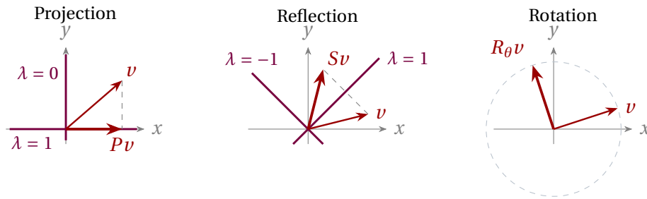
Figure 2: The projection P onto the x axis, the reflection S across the line y = x , and the rotation R_\theta . The highlighted lines are the eigendirections, labelled with their eigenvalues. The vector v is not an eigenvector, so its image is not parallel to it. When \theta \notin \pi\mathbb{Z} , a rotation moves every nonzero real vector off its line, so there are no real eigenvectors.
