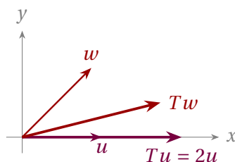
Figure 1: The eigendirection of the transformation T(x, y) = (2x, \frac{1}{2}y) is the x axis: Tu = 2u . A general vector w is turned, so it is not an eigenvector.
