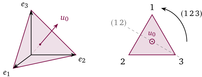
Figure 4.2: Left: the tips of e_1, e_2, e_3 span an equilateral triangle perpendicular to u_0 . Right: its projection onto V_0 , seen down u_0 . The cycle (1\ 2\ 3) rotates it through 2\pi/3 . The transposition (1\ 2) reflects it in the dashed axis.
