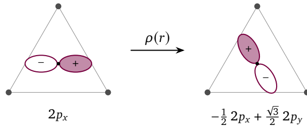
Figure 4.3: Left: the orbital 2p_x of an atom at the centre of the triangle. Right: the rotation r turns it through 2\pi/3 , into a superposition of 2p_x and 2p_y .
