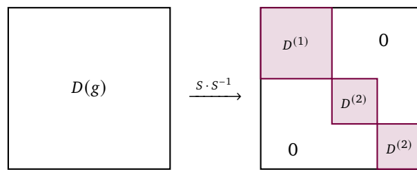
Figure 4.1: Maschke's theorem in matrix form: a single change of basis S brings every D(g) , for all g \in G at once, to the same block-diagonal form with irreducible blocks. Blocks may repeat: here the irreducible representation D^{(2)} occurs with multiplicity two.
