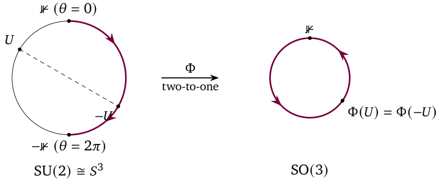
Figure 11.1: The double cover. Left: a great circle \theta \mapsto e^{-i\theta\sigma_3/2} of SU(2) \cong S^3 ; as \theta runs from 0 to 2\pi it traces the accented open path from I to -I — half the circle, the halved angle at work. Right: its image under \Phi , the closed loop R_z(\theta) in SO(3) , traversed once in full. Antipodal points \pm U (dashed chord) share a single image: \Phi glues opposite points of the sphere. The open lift is the obstruction of Proposition 11.3 — contracting the loop downstairs would have to drag the lift's endpoint through the discrete fibre \{\pm I\} — while doubling the range to 4\pi closes the lift, which then contracts in S^3 .
