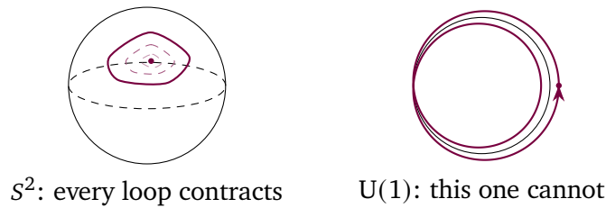
Figure 9.1: Two topologies for loops. On the sphere every loop shrinks through intermediate loops (dashed) to its basepoint; the same holds on S^3 , though that picture resists printing. On the circle a loop that winds twice — drawn slightly off the circle so that both passes are visible — can never contract: its winding number is pinned.
