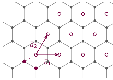
Figure 2.2: The honeycomb. Grey dots are carbon atoms; open circles mark the cell origins, taken here at the hexagon centres, where there is no atom; the vectors between any two of them are exactly the lattice \Lambda . The two filled atoms are the motif carried by the marked lattice point — one from each sublattice — and translating that pair through \Lambda produces every atom. The atoms themselves do not form a lattice.
