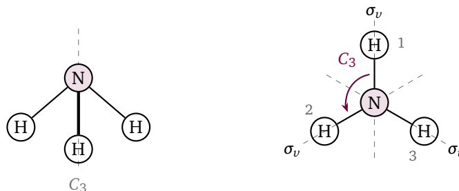
Figure 5.1: The ammonia molecule \text{NH}_3 . On the left it is seen from the side (the thick bond points towards the reader), on the right from above, down the axis C_3 . The dashed lines on the right are the three mirror planes \sigma_v , and the arrow is the rotation through 2\pi/3 , which takes hydrogen 1 to the place of hydrogen 2.
