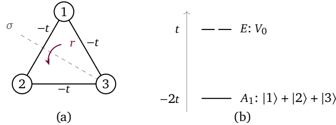
Figure 6.1: The particle on a triangle. (a) One orbital |j\rangle on each atom j , and the hopping amplitude -t on each bond. The rotation r takes atom 1 to the place of atom 2. The mirror \sigma (the dashed line) fixes atom 3 and swaps atoms 1 and 2. (b) The two energy levels, drawn for t > 0 : the singlet A_1 at -2t and the doublet E at t .
