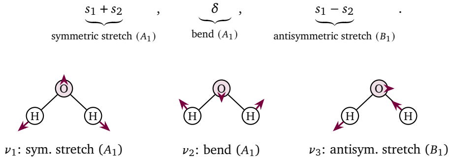
Figure 6.1: The three normal modes of water with their Mulliken labels. Small arrows on the oxygen keep the centre of mass fixed. The two A_1 coordinates mix; the patterns shown are the symmetry-adapted coordinates whose 2 \times 2 reduced matrix determines the two A_1 frequencies.
