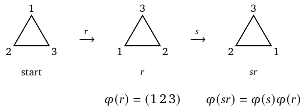
Figure 1.5: Performing r and then s gives the same result as applying sr at once. The labels travel with the triangle, so the permutations multiply in the same order.
