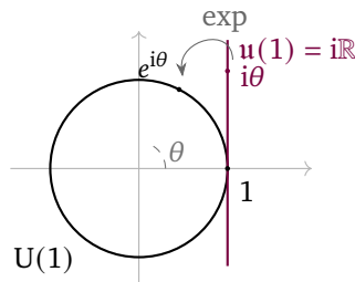
Figure 8.1: The exponential map of the circle group: \exp wraps the tangent line u(1) = i\mathbb{R} around \text{U}(1) with period 2\pi — bijective near the identity, not injective globally, surjective onto the connected compact group.
