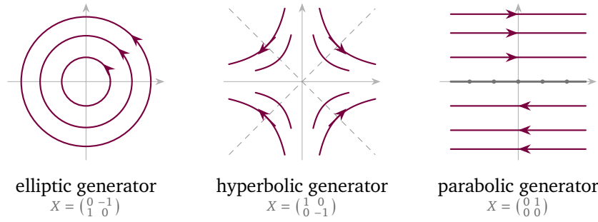
Figure 8.2: Three qualitative generator types in \mathfrak{sl}(2, \mathbb{R}) , drawn through their flows t \mapsto e^{tX} on the plane. For the displayed elliptic representative, \text{tr}(e^{tX}) = 2 \cos t : it reaches the central elements \pm \mathbb{I} when t \in \pi\mathbb{Z} and has |\text{tr}(e^{tX})| < 2 otherwise. For the displayed hyperbolic representative, \text{tr}(e^{tX}) = 2 \cosh t : it is \mathbb{I} at t = 0 and has trace greater than 2 otherwise. For the displayed parabolic representative, e^{tX} = \mathbb{I} + tX has trace 2; it is the identity at t = 0 and a nontrivial shear otherwise. Thus these pictures organise flow behaviour, not the individual conjugacy classes: the zero generator and central group elements are exceptional, each qualitative type contains further conjugacy data, and signs/orientations — notably X versus -X for a nilpotent generator inside \text{SL}(2, \mathbb{R}) — are not encoded by the drawings.
