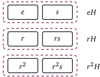
Figure 1.6: Splitting D_3 into the left cosets of the subgroup H = \langle s \rangle = \{e, s\} . All six elements fall into three blocks. The blocks are disjoint, each holds |H| = 2 elements, and together they exhaust the group. This is exactly what Lagrange's theorem says: |D_3| = 3 \cdot 2 .
