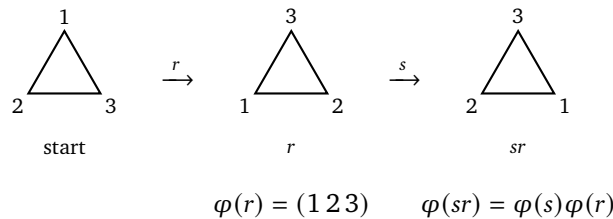
Figure 1.5: Why \varphi preserves multiplication. Performing r and then s gives the same result as applying sr at once. The labels travel with the triangle, so the permutations multiply in the same order.
