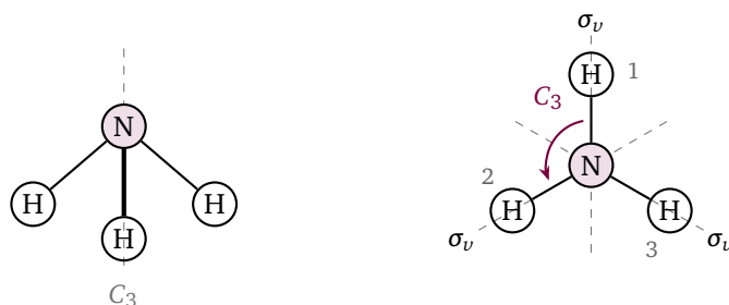
Figure 5.1: The ammonia molecule \text{NH}_3 . On the left it is seen from the side (the thick bond points towards the reader), on the right from above, down the axis C_3 . The dashed lines on the right are the three mirror planes \sigma_v , and the arrow is the rotation through 2\pi/3 , which takes hydrogen 1 to the place of hydrogen 2.
