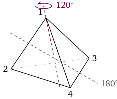
Figure 2.5: The regular tetrahedron with numbered vertices. The rotation by 120^\circ about the axis through vertex 1 and the centre of the opposite face permutes the other three vertices cyclically: a 3-cycle. The half-turn about the axis through the midpoints of edges 12 and 34 swaps 1 \leftrightarrow 2 and 3 \leftrightarrow 4 : it is (1\ 2)(3\ 4) .
