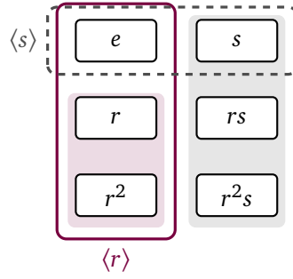
Figure 2.3: The two partitions of D_3 in one picture. The rows are the cosets of \langle s \rangle , the columns the cosets of \langle r \rangle , and the shaded regions are the conjugacy classes \{e\} , \{r, r^2\} and \{s, rs, r^2s\} . The subgroup \langle r \rangle (solid outline) is made of whole classes, so it is normal. The subgroup \langle s \rangle (dashed outline) cuts across the class of reflections, so it is not.
