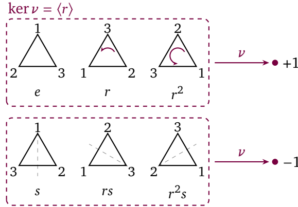
Figure 2.1: The orientation homomorphism \nu: D_3 \rightarrow \{\pm 1\} . All three rotations (top) go to +1 and all three reflections (bottom) to -1 : each dashed block is collapsed to a single point, and the top block is the kernel. Under the isomorphism D_3 \cong S_3 this is the sign \text{sgn} : the rotations are the even permutations, the reflections the odd ones.
