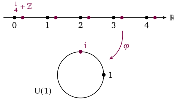
Figure 2.4: Winding the real line onto the circle, \varphi(x) = e^{2\pi ix} . All integers (black) go to 1, all points of \frac{1}{4} + \mathbb{Z} (coloured) go to i . Each coset x + \mathbb{Z} becomes a single point of the circle, so \mathbb{R}/\mathbb{Z} \cong U(1) .
