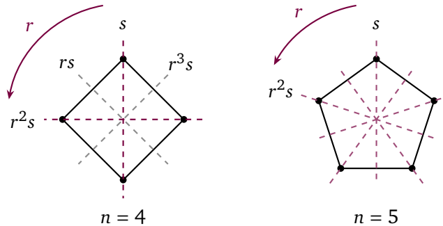
Figure 2.2: Conjugation by the rotation r in D_4 and D_5 . A mirror axis turns through the same angle 2\pi/n as r , but neighbouring axes are only \pi/n apart, so the index of the reflection goes up by two: rsr^{-1} = r^2s . In the square an axis through vertices (coloured) therefore always goes to an axis through vertices, and an axis through edge midpoints (grey) to another of its kind: the reflections split into two classes. In the pentagon the rotations reach all five axes, and there is one class.
