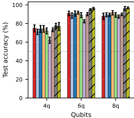
Fashion-MNIST
