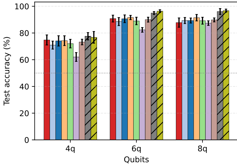
Fashion-MNIST
