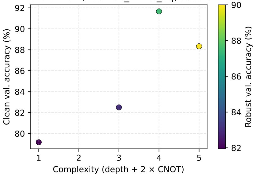
Pareto front, fashion_mnist_6q, seed 0
