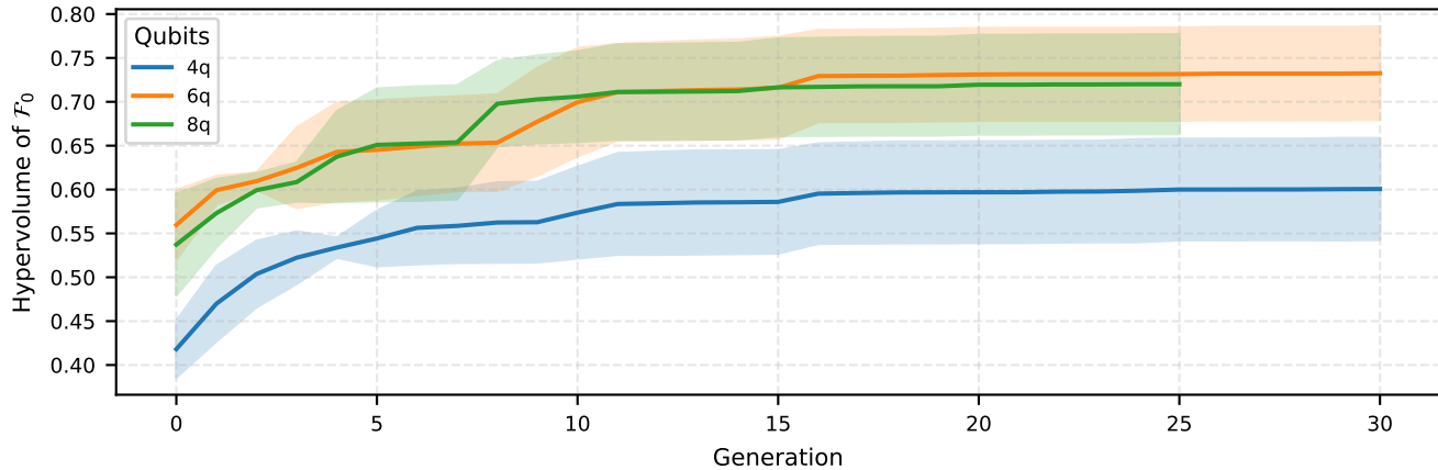
Fashion-MNIST
