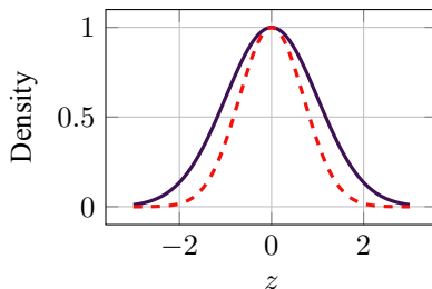
Figure 19.2: Mean field (dashed) often underestimates posterior variance (illustrative).
