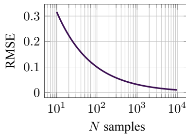
Figure 17.1: Monte Carlo error decreases as \mathcal{O}(N^{-1/2}) (illustrative).
