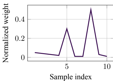
Figure 17.3: Weight degeneracy: a few samples dominate (illustrative).
