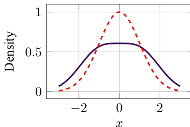
Figure 19.4: EP (solid) can better match multi-modal targets than simple mean-field Gaussian (dashed), illustrative.
