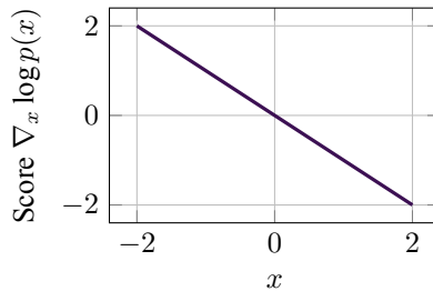
Figure 18.4: Score function for a standard normal p(x) \propto e^{-x^2/2} is -x (illustrative).
