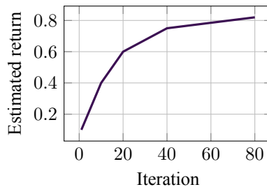
Figure 17.4: Monte Carlo return estimates improving with more rollouts (illustrative).
