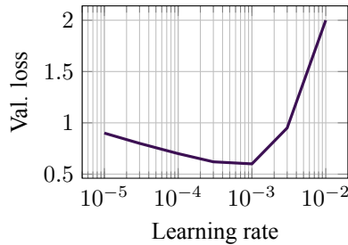
Figure 11.9: Learning-rate sweep identifies a stable operating region.
