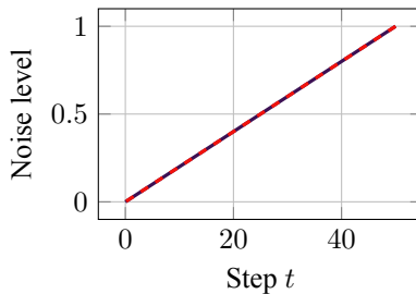
Figure 20.4: Forward (solid) and reverse (dashed) diffusion noise schedules (illustrative).
