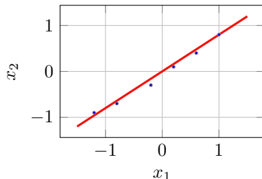
Figure 13.1: PCA principal axis capturing maximum variance.
