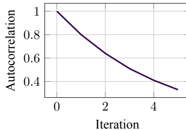
Figure 17.2: Autocorrelation decay in an MCMC chain (illustrative).
