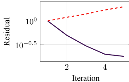
Figure 19.3: Loopy BP: a convergent case (solid) vs. a divergent case (dashed), illustrative.
