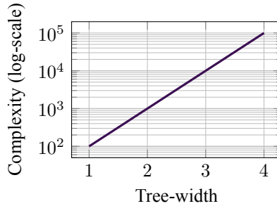
Figure 16.3: Exact inference complexity grows rapidly with tree-width (illustrative).
