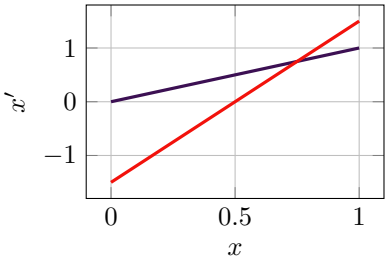
Figure 11.11: Min-max scaling (purple) vs. standardization (red) schematic.
