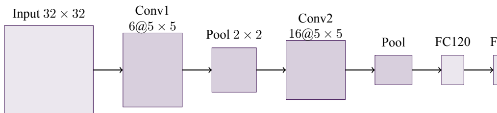
Figure 9.3: LeNet-5 architecture: alternating conv and pooling, followed by small fully connected layers.
