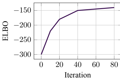
Figure 19.1: ELBO increasing during variational optimization (illustrative).
