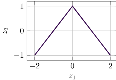
Figure 13.4: Schematic illustrating \ell_1 -induced sparsity geometry.
