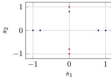
Figure 13.3: Independent sparse sources aligned with axes (illustrative).
