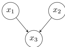
Figure 16.1: A simple Bayesian network (DAG) encoding conditional dependencies.
