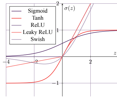
Figure 6.2: Comparison of common activation functions. Each function has different properties: sigmoid and tanh saturate at extreme values, ReLU is simple but can “die”, while Swish provides smooth gradients.
