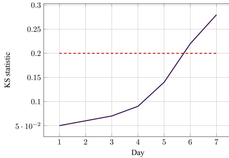
Figure 11.12: Simple drift monitor: KS statistic over time with an alert threshold.
