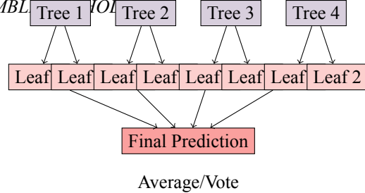
Figure 5.8: Random forests combine multiple decision trees. Each tree is trained on a different bootstrap sample and makes its own prediction. The final prediction is the average (regression) or majority vote (classification) of all trees.
