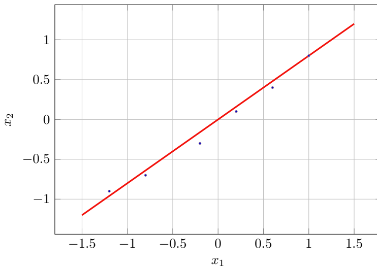
Figure 13.1: PCA principal axis capturing maximum variance.
