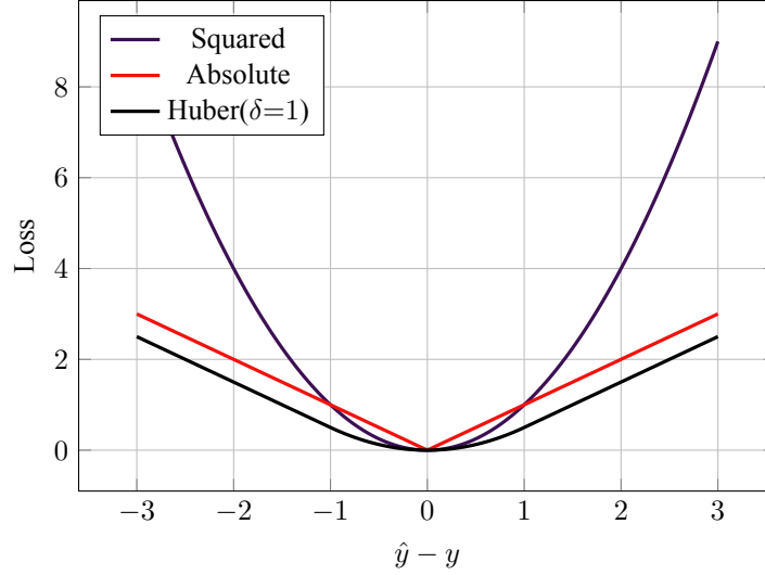
Figure 11.5: Comparison of squared, absolute, and Huber losses.
