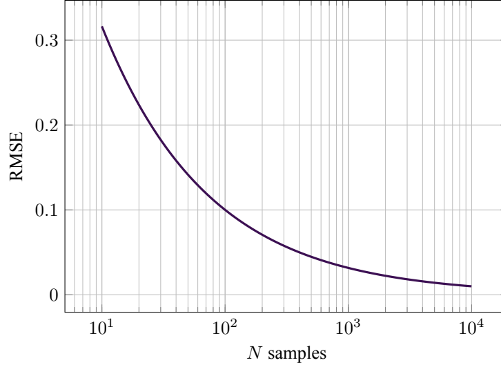
Figure 17.1: Monte Carlo error decreases as \mathcal{O}(N^{-1/2}) (illustrative).
