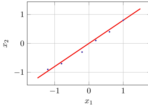
Figure 13.1: PCA principal axis capturing maximum variance.
