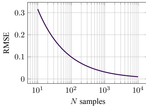
Figure 17.1: Monte Carlo error decreases as \mathcal{O}(N^{-1/2}) (illustrative).
