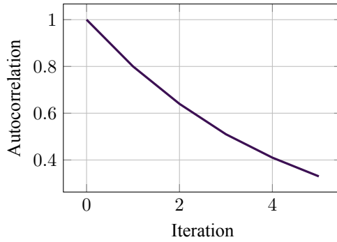
Figure 17.2: Autocorrelation decay in an MCMC chain (illustrative).
