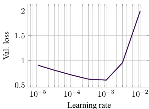
Figure 11.9: Learning-rate sweep identifies a stable operating region.
