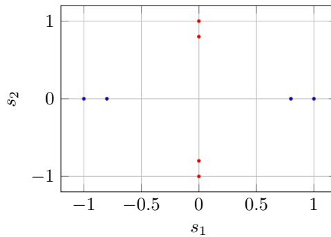
Figure 13.3: Independent sparse sources aligned with axes (illustrative).
