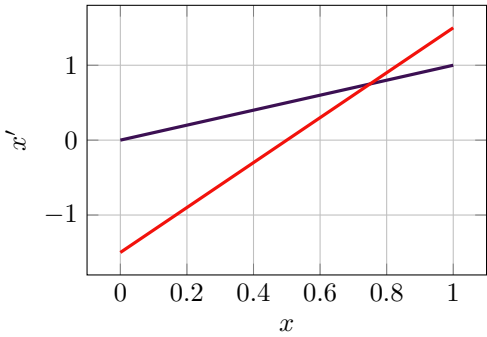
Figure 11.11: Min-max scaling (purple) vs. standardization (red) schematic.
