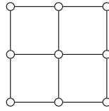
Figure 16.2: Undirected MRF grid with pairwise potentials between neighbors.
