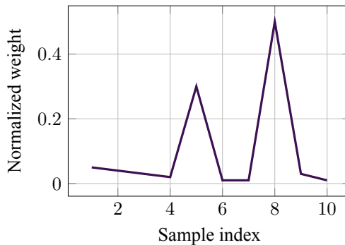
Figure 17.3: Weight degeneracy: a few samples dominate (illustrative).
