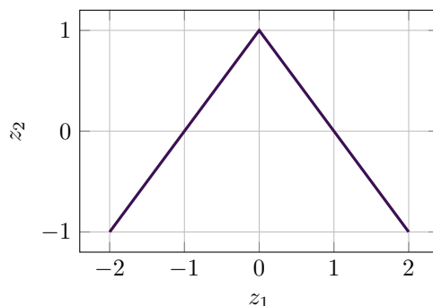
Figure 13.4: Schematic illustrating \ell_1 -induced sparsity geometry.
