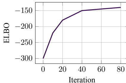
Figure 19.1: ELBO increasing during variational optimization (illustrative).
