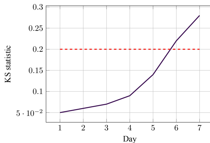
Figure 11.12: Simple drift monitor: KS statistic over time with an alert threshold.
