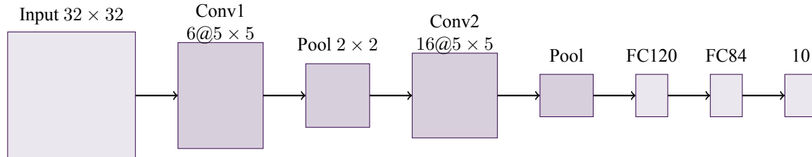
Figure 9.3: LeNet-5 architecture: alternating conv and pooling, followed by small fully connected layers.
