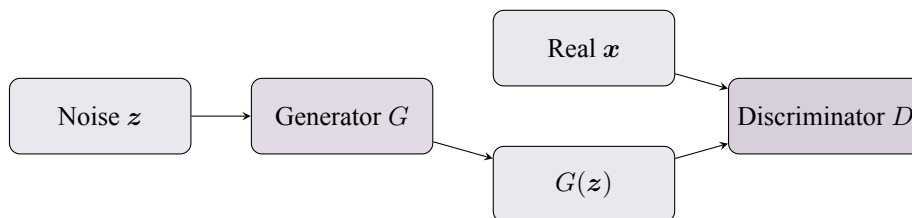
Figure 20.2: GAN training: generator produces samples to fool discriminator.
