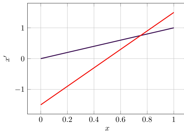
Figure 11.11: Min-max scaling (purple) vs. standardization (red) schematic.
