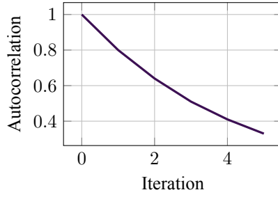
Figure 17.2: Autocorrelation decay in an MCMC chain (illustrative).
