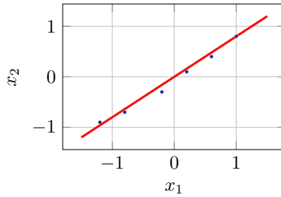
Figure 13.1: PCA principal axis capturing maximum variance.
