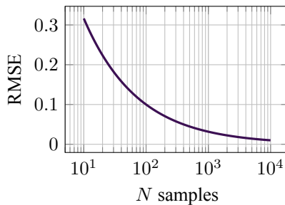
Figure 17.1: Monte Carlo error decreases as \mathcal{O}(N^{-1/2}) (illustrative).
