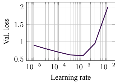
Figure 11.9: Learning-rate sweep identifies a stable operating region.
