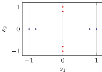
Figure 13.3: Independent sparse sources aligned with axes (illustrative).
