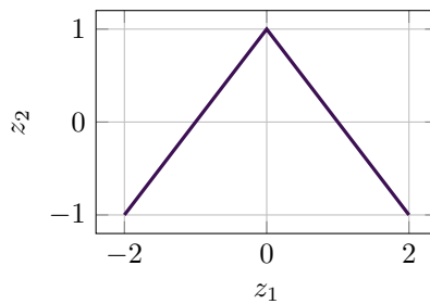
Figure 13.4: Schematic illustrating \ell_1 -induced sparsity geometry.
