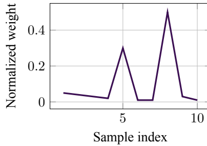
Figure 17.3: Weight degeneracy: a few samples dominate (illustrative).
