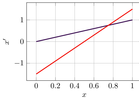
Figure 11.10: Min-max scaling (purple) vs. standardization (red) schematic.
