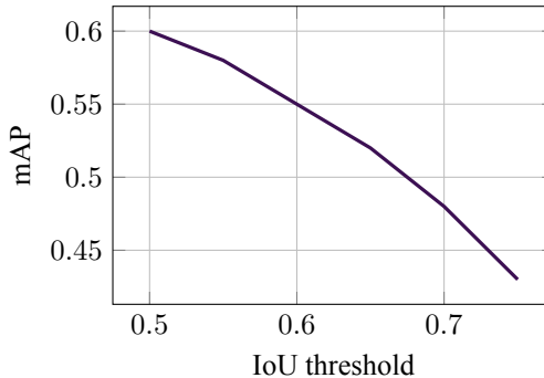
Figure 12.2: Detector performance (mAP) vs. IoU threshold schematic.
