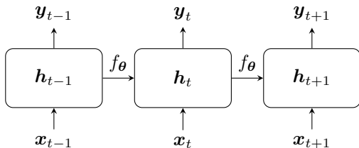
Figure 10.2: Unrolling an RNN across time: the same parameters \boldsymbol{\theta} are reused at each step.
