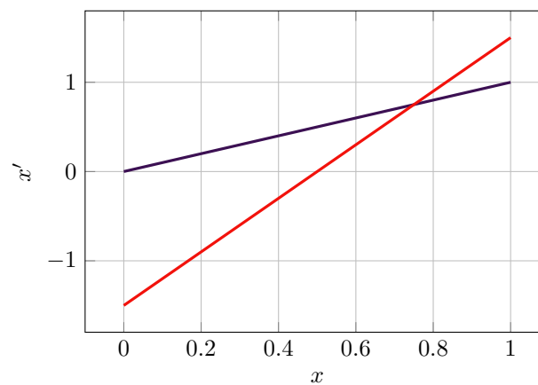
Figure 11.10: Min-max scaling (purple) vs. standardization (red) schematic.
