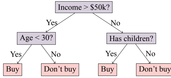
Figure 5.7: A simple decision tree for predicting product purchases. Each internal node represents a decision, and leaf nodes represent the final prediction.
