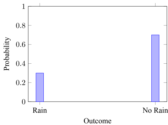
Figure 3.1: Probability distribution for rain prediction
