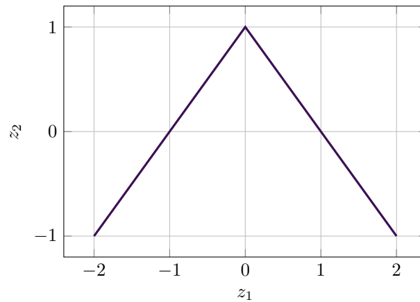
Figure 13.2: Schematic illustrating \ell_1 -induced sparsity geometry.
