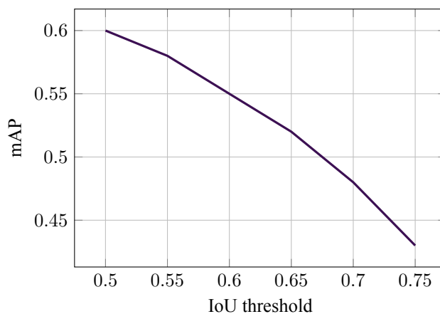
Figure 12.2: Detector performance (mAP) vs. IoU threshold schematic.
