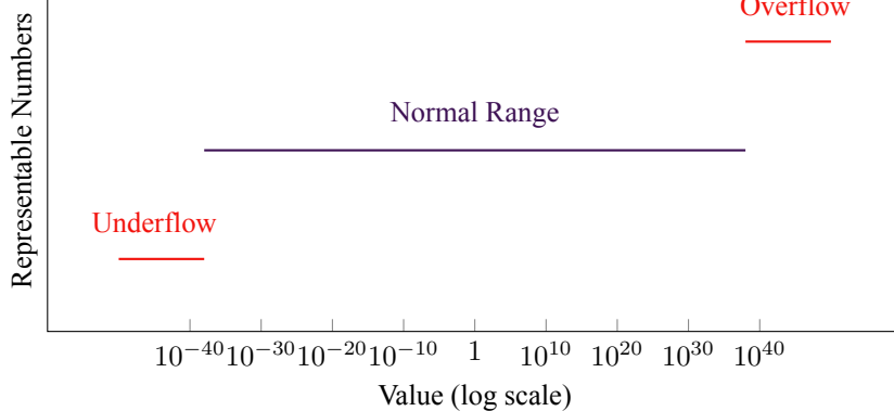
Figure 4.1: Representable range for 32-bit floating-point numbers
