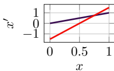
Figure 11.11: Min-max scaling (purple) vs. standardization (red) schematic.
