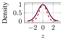
Figure 19.2: Mean field (dashed) often underestimates posterior variance (illustrative).
