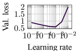
Figure 11.9: Learning-rate sweep identifies a stable operating region.
