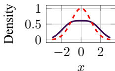
Figure 19.4: EP (solid) can better match multi-modal targets than simple mean-field Gaussian (dashed), illustrative.
