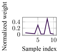
Figure 17.3: Weight degeneracy: a few samples dominate (illustrative).
