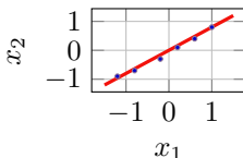
Figure 13.1: PCA principal axis capturing maximum variance.
