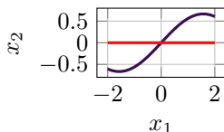
Figure 15.1: Complex data manifold (purple) and a learned linearized coordinate (red) locally.
