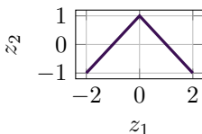
Figure 13.4: Schematic illustrating \ell_1 -induced sparsity geometry.
