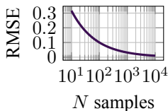
Figure 17.1: Monte Carlo error decreases as \mathcal{O}(N^{-1/2}) (illustrative).
