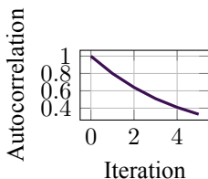
Figure 17.2: Autocorrelation decay in an MCMC chain (illustrative).
