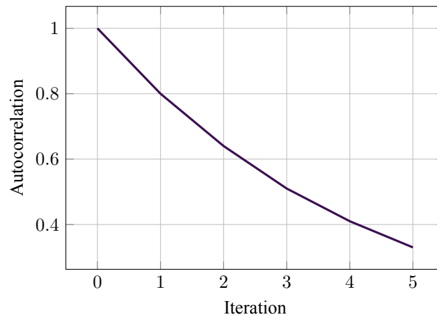
Figure 17.2: Autocorrelation decay in an MCMC chain (illustrative).
