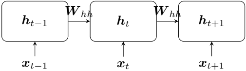
Figure 10.1: Unrolled RNN with shared parameters across time steps.
