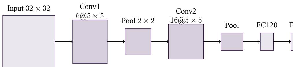
Figure 9.2: LeNet-5 architecture: alternating conv and pooling, followed by small fully connected layers.
