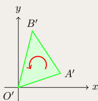
\det(M_k) > 0 (Preserves orientation)
