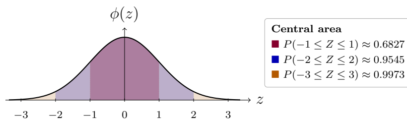
Figure: the standard normal curve with the central one-, two-, and three-standard-deviation regions shaded.
