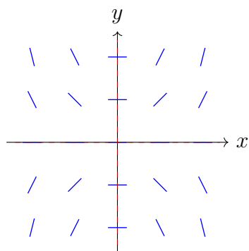
Example 1: y' = xy
