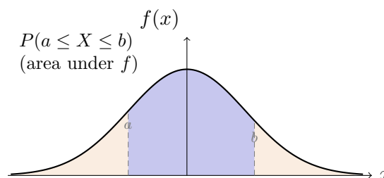
Probability for a continuous X : the shaded interval has P(a \leq X \leq b) = \int_a^b f(x) dx ; point masses have probability 0.
