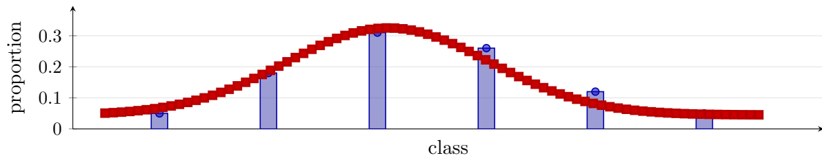
Relative frequencies bar-chart a distribution; narrower bins with more data approach a smooth curve (pdf analogue).
