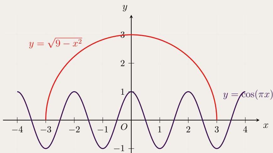
Figure 2: Graphs of f(x) = \cos(\pi x) and g(x) = \sqrt{9 - x^2}
