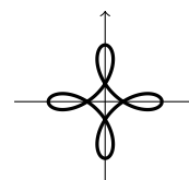
Hypotrochoid
