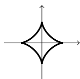
Hypocycloid
