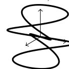
3D Lissajous Curve
