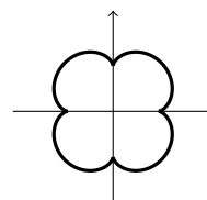
Epicycloid
