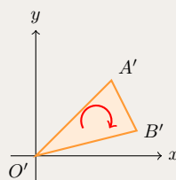
\det(M_k) < 0 (Reverses orientation)
