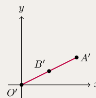
\det(M_k) = 0 (Collapses to 1D)
