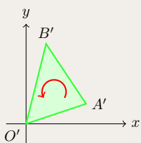
\det(M_k) > 0 (Preserves orientation)
