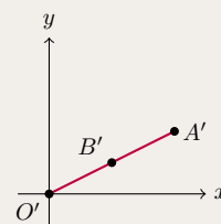
\det(M_k) = 0 (Collapses to 1D)
