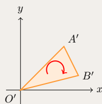
\det(M_k) < 0 (Reverses orientation)
