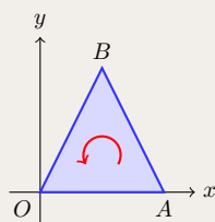
Original T (CCW)
