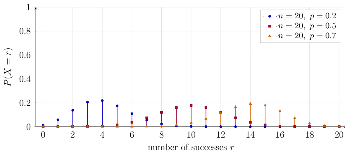
Figure: binomial probability mass functions for X \sim B(20, p) . As p increases, the distribution shifts to the right because the expected number of successes is np .
