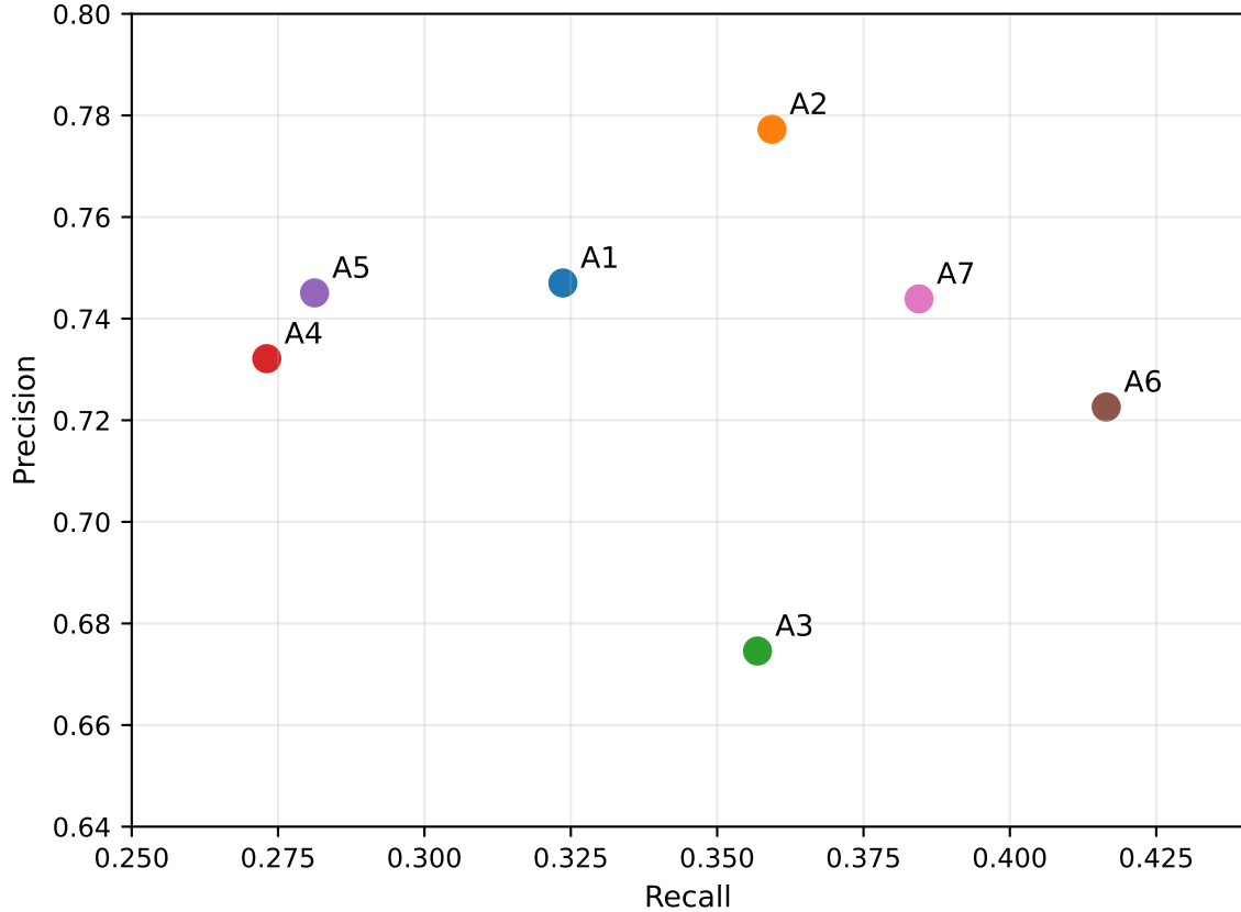
Precision-recall trade-off across ablations
