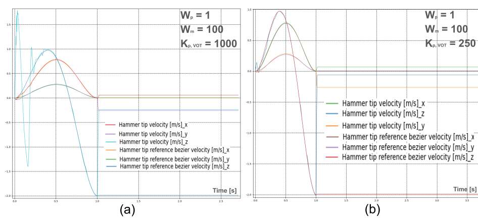
Fig. 3. Velocity tracking of the hammer tip for different K_{p,VOT} values
