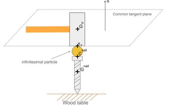
Fig. 1. Schematic of the collision using particle impact
