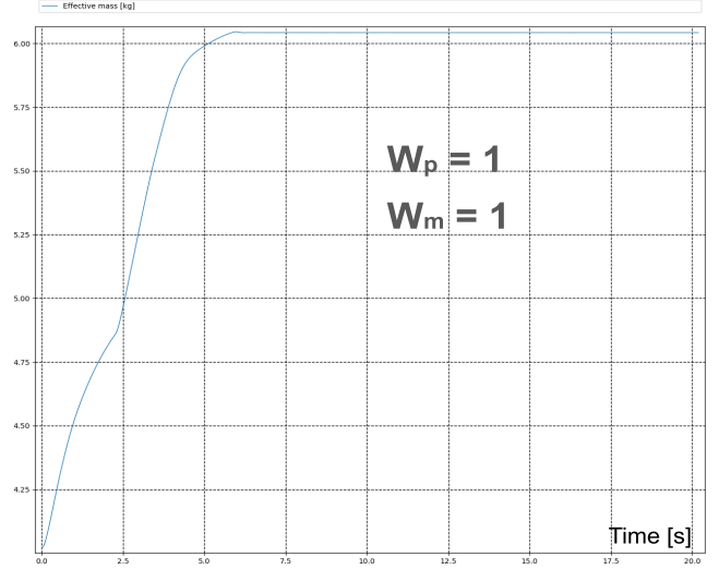
Fig. 2. Time evolution of the EMR with only a posture task active
