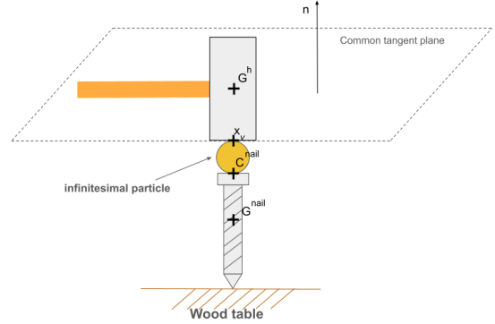
Fig. 1. Schematic of the collision between the hammer tip and the nail modeled as a particle impact
